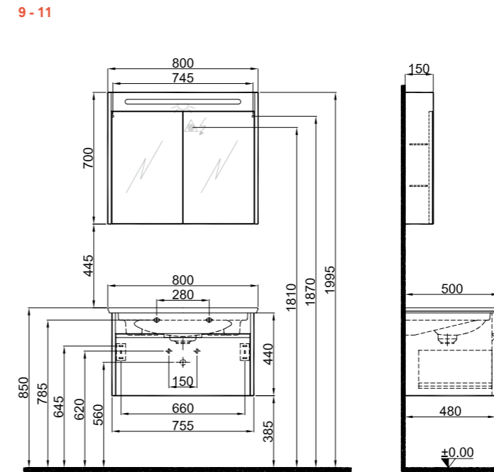
80 cm Set Front and Side View
