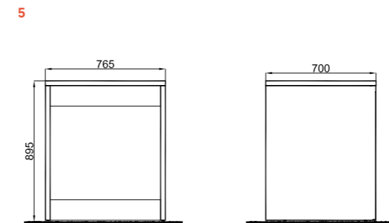
76 cm Washing Machine Cabinet (Without Doors) Front and Side View
