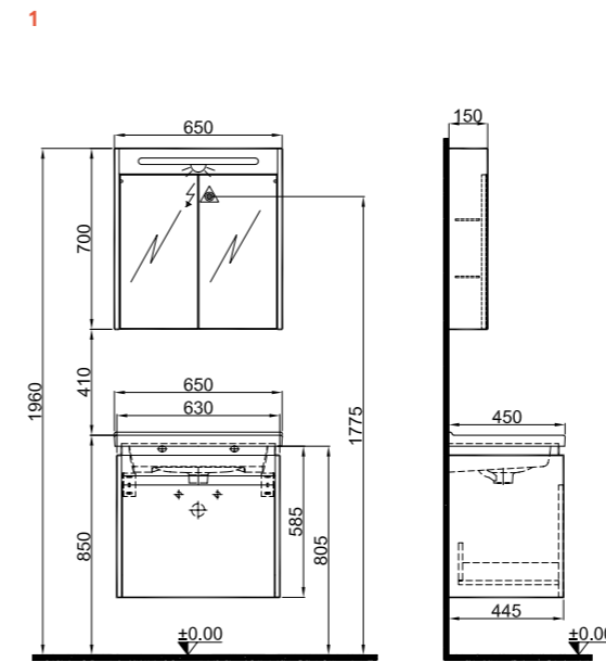
65 cm Set with Single Drawer Front and Side
