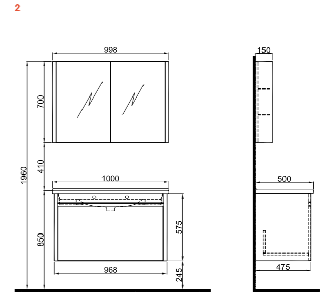
100 cm Set Front and Side View
