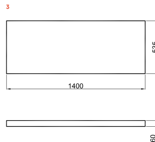
140 cm Shelf Front and Side View
