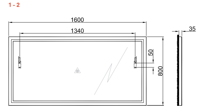
160 x 80 cm Mirror Front and Side View
