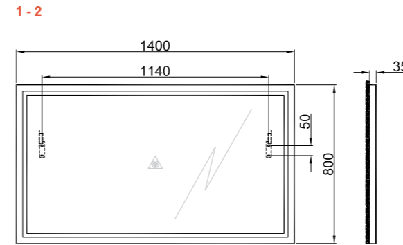
140 x 80 cm Mirror Front and Side View
