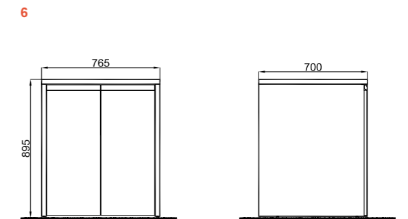
76 cm Washing Machine Cabinet (With Door) Front and Side View
