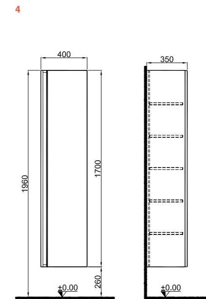
40 cm Tall Cabinet Front and Side View
