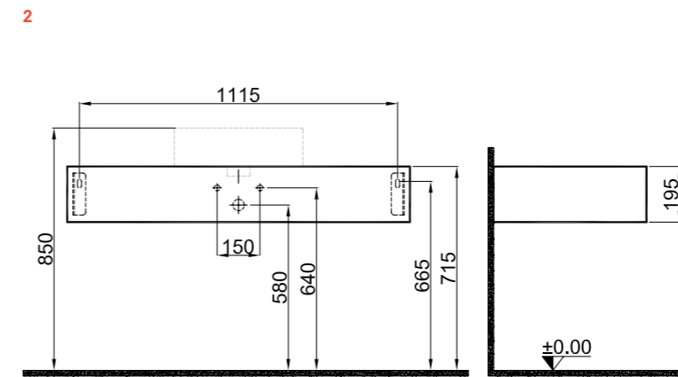
K2 120 cm Sinterflex Counter Washbasin Front and Side View
