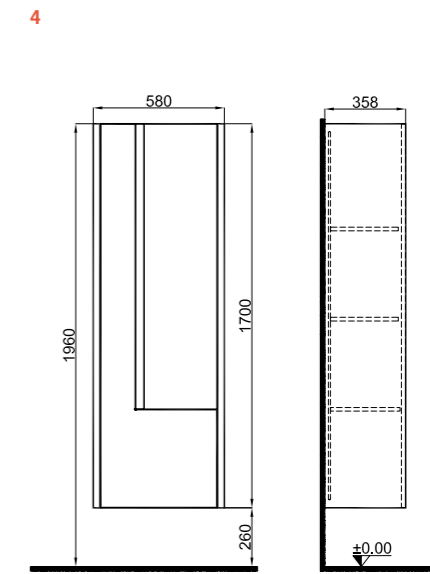
58 cm Tall Cleaning Cabinet Front and Side View
