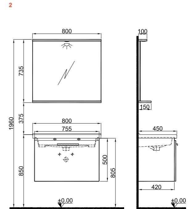
80 cm Set Front and Side View
