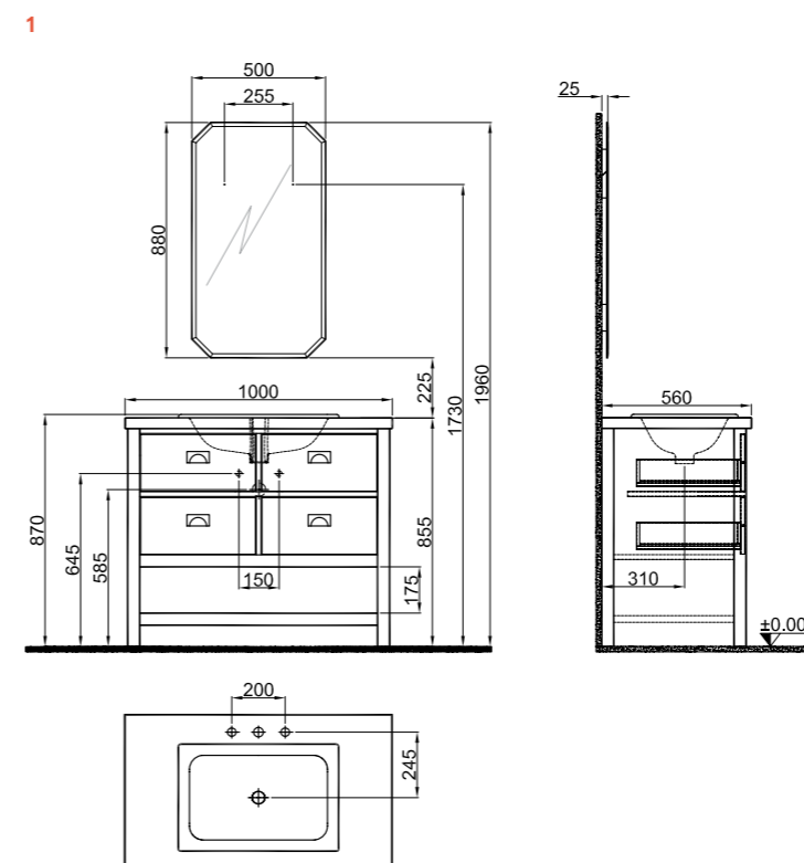
100 cm Set Front and Side View
