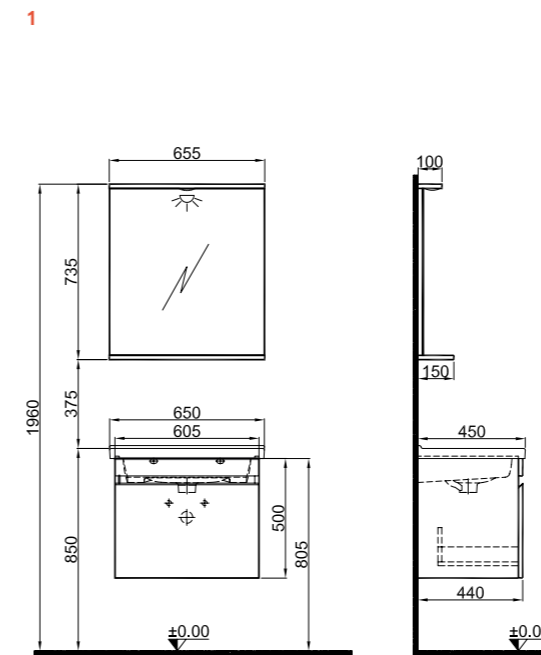
65 cm Set Front and Side View
