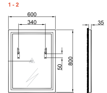
60 x 80 cm Mirror Front and Side View
