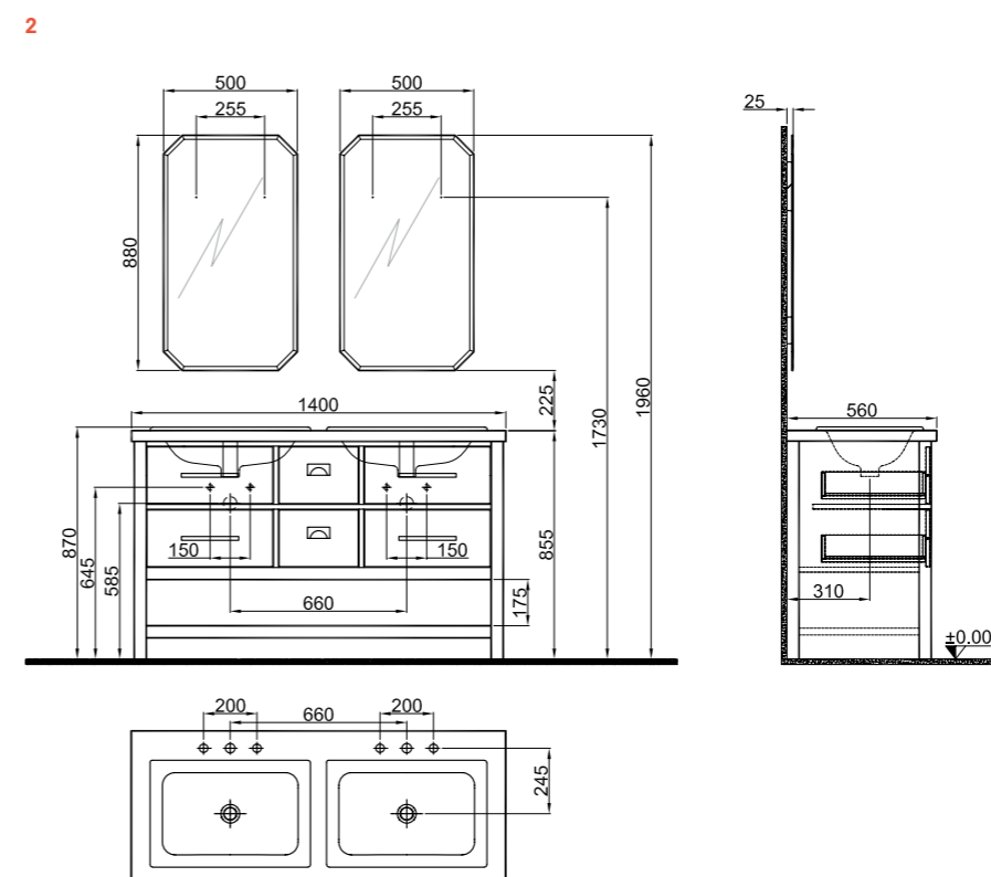
140 cm Set Front and Side View
