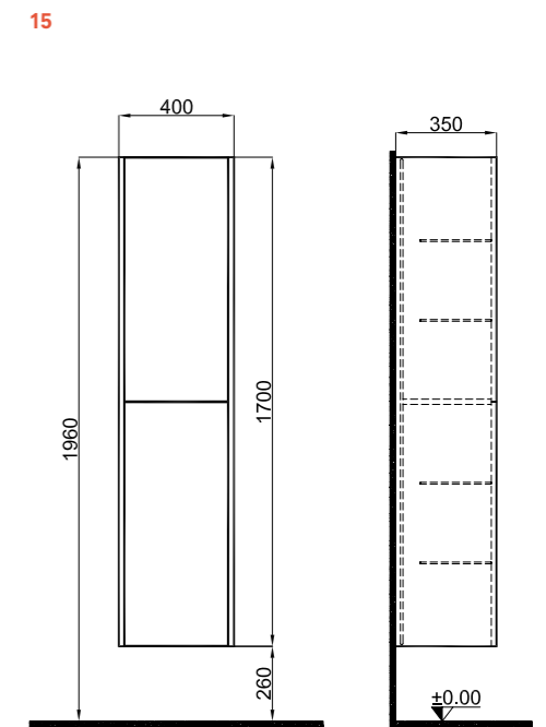
50 cm Tall Cabinet Front and Side View
