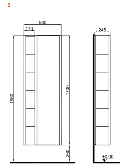
58 cm Tall Cabinet Front and Side View
