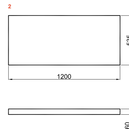
120 cm Shelf Front and Side View
