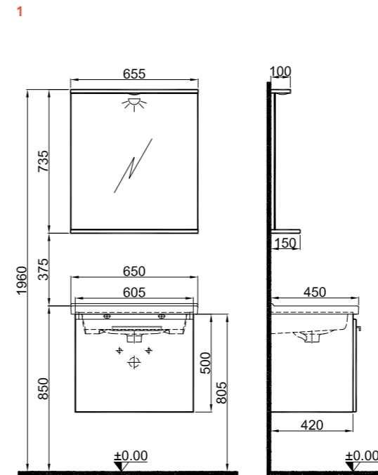
65 cm Set Front and Side View
