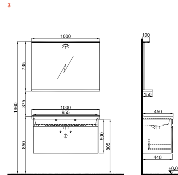
100 cm Set Front and Side View
