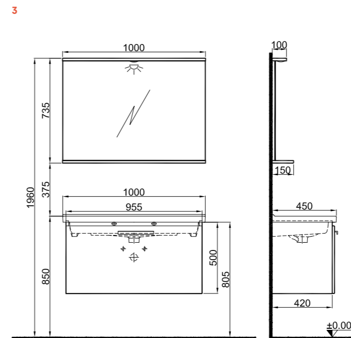
100 cm Set Front and Side View
