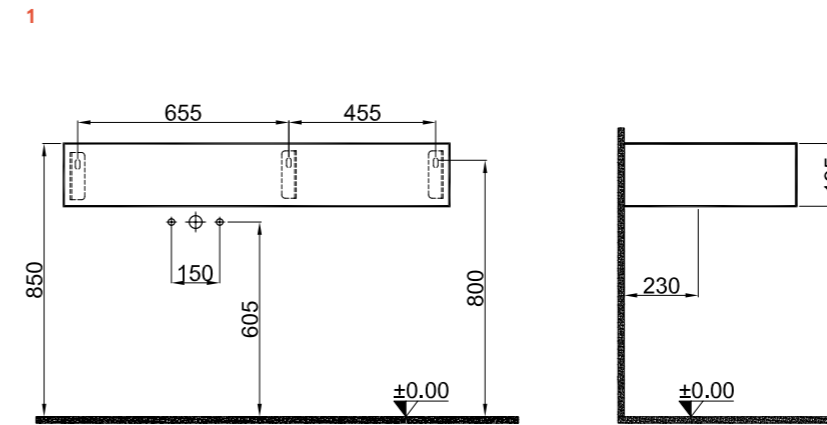
K1 120 cm Sinterflex Counter Washbasin Front and Side View
