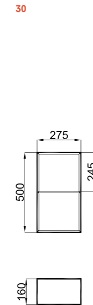
Open Top Shelf Module 28 cm Front and Side View
